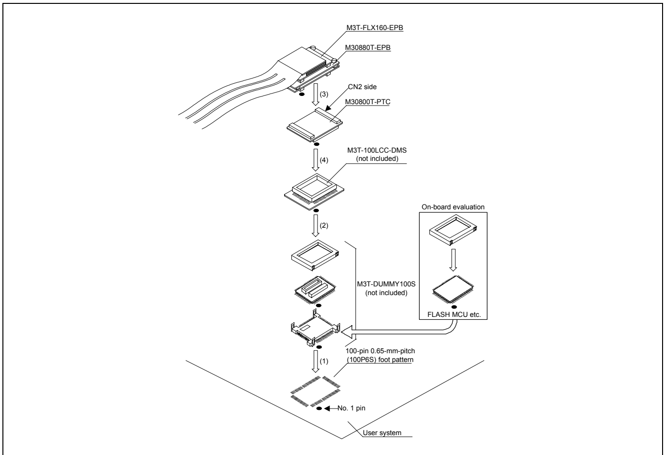
Figure 2.9 Connecting to a 100-pin 0.65-mm-pitch foot pattern (1/3)
